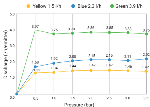
PoliDrip PC Ø20 mm
