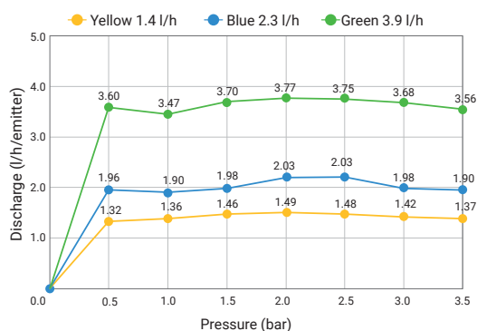
PoliDrip PC Ø16 mm
